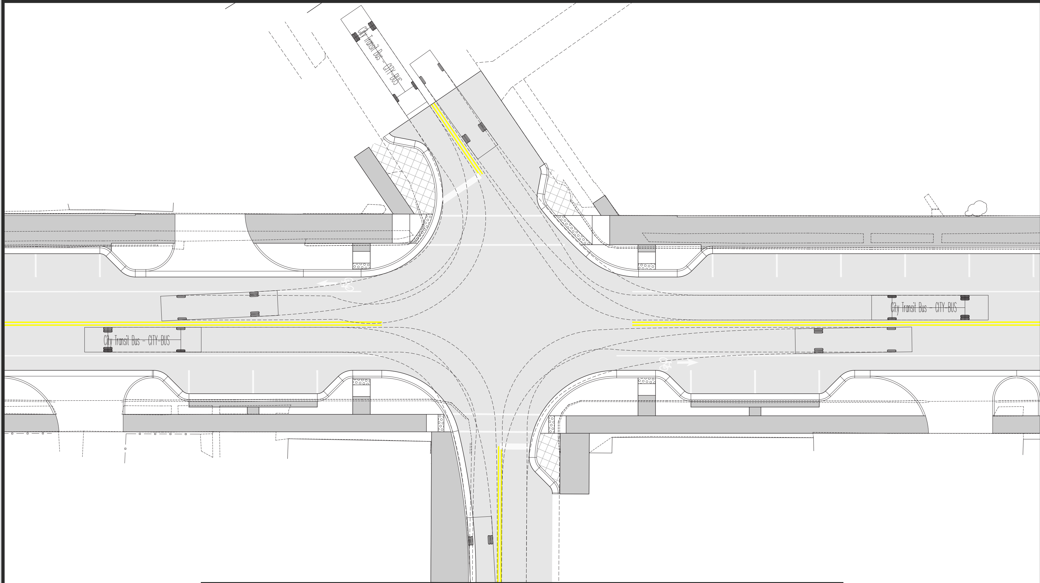
FIRE TRUCK, SCHOOL BUS, WB-50 NO LANE ENCROACHMENT
